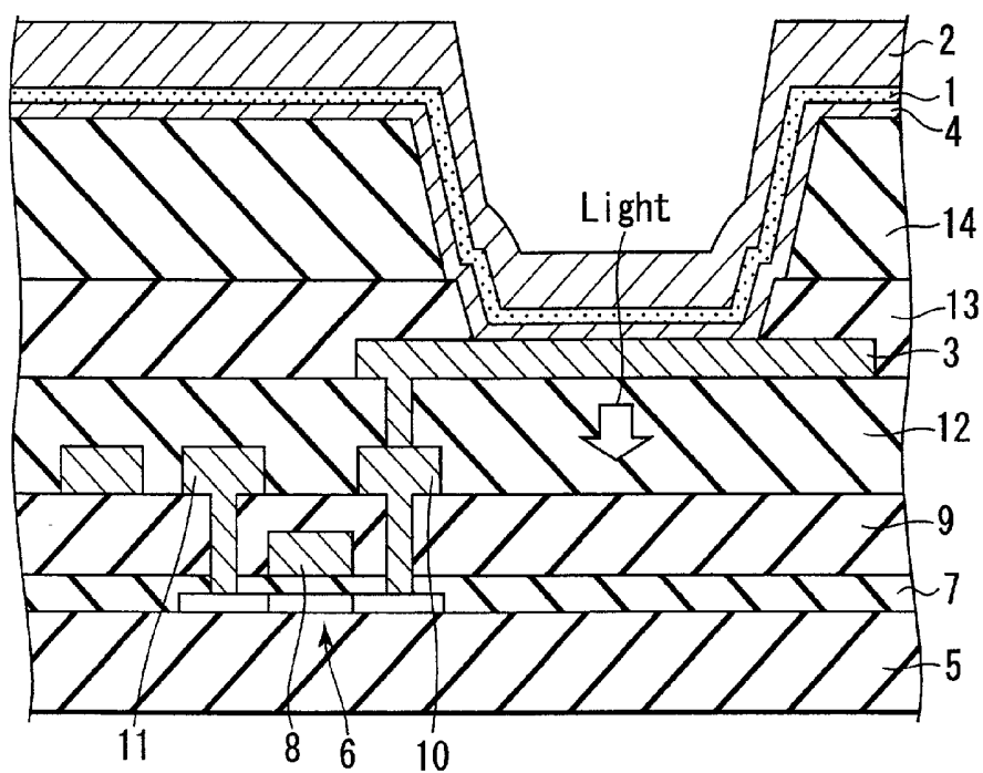
FIG. 5 (PRIOR ART)
